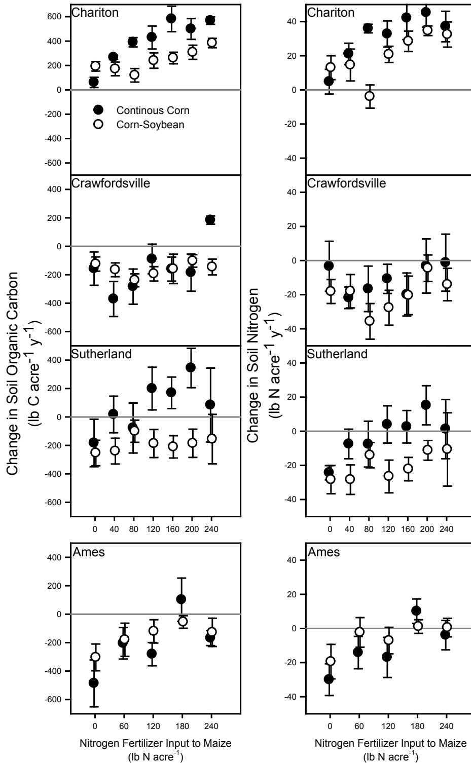
Figure 5. Average annual rate of change of soil organic carbon and total soil nitrogen stocks in the top 7.87" (15 cm) of soil over 10 years at Ames, Chariton, and Carwafordsvile and over 9 years at Sutherland. Error bars represent standard error. N = 4 replicated plots for continuous corn, N = 8 replicated plots for corn-soybean. 1 kg per hectare = 0.89 pounds per acre. Open circles are corn-soybean rotation, closed circles are continuous corn. Symbols are offset for visual clarity.
