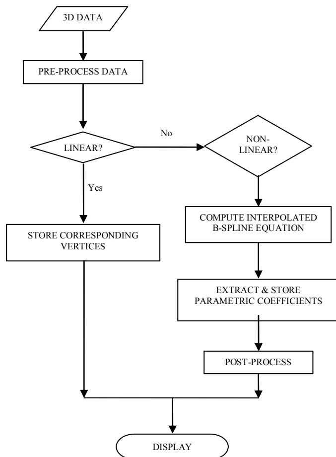
Figure 1 - Methodology outline
