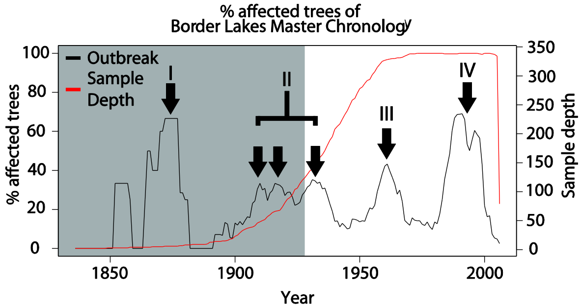
Figure 2: Master chronology for the full BLL study area. The grey section was excluded from formal analyses due to low sample size at the level of the sample unit (ie., subarea). Sample depth (red line) refers to the number of trees upon which the disturbance chronology (percent affected trees; black line) is based. Cycle peaks associated with four major cycles (I-IV) are indicated with arrows.
