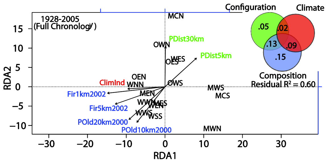
Figure 6: Redundancy Analysis (RDA) and variance partitioning relating dissimilarity in the annual percent trees affected to independent variables chosen by forward selection for each of our three hypotheses: (1) forest configuration; (2) forest composition; and (3) climate. See Table 1 for subarea acronyms in black font. Inset bubble diagrams indicate the independent and shared variance explained by each class of variables (see Table 2 for predictor variable descriptions, where the color label corresponds to the class of variables in the bubble diagram). The RDA is applied to the full chronology is contrasted with separate RDAs applied to each of the three major outbreak periods (Fig. 7).
