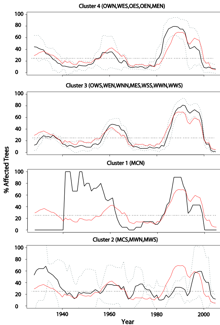
Figure 4: Combined chronologies for each of the four clusters shown in Figure 3, listed from the southwest (bottom) to the northeast (top). Black = average percentage of trees affected for the cluster. Dashed gray = 95% confidence intervals for the cluster. Red = average percentage of trees affected for the entire study area (Fig. 1). Dotted horizontal line indicates the 25% threshold defining outbreaks in prior study (Robert et al. 2012) – but this line is used for reference only and not applied in any analysis. Difference between red and black curves shows the deviation of a cluster from the broader BLL temporal pattern. See Table 1 for subarea acronyms, and Appendix 2 for raw subarea-level chronologies. Spectral peak from spectral analysis is the following for each Cluster: Cluster 4 & 3: 33 years, Cluster 2: 12-15 years, Cluster 1: 44 years
