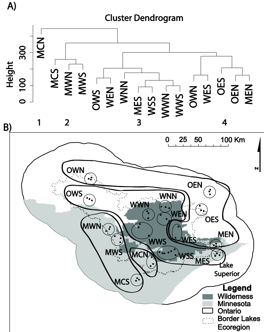
Figure 3: A. Results of the cluster analysis (n = 4) of the percentage of trees affected by defoliation in the 16 subareas. B. The four clusters overlaid in geographical space. See Table 1 for subarea acronyms.
