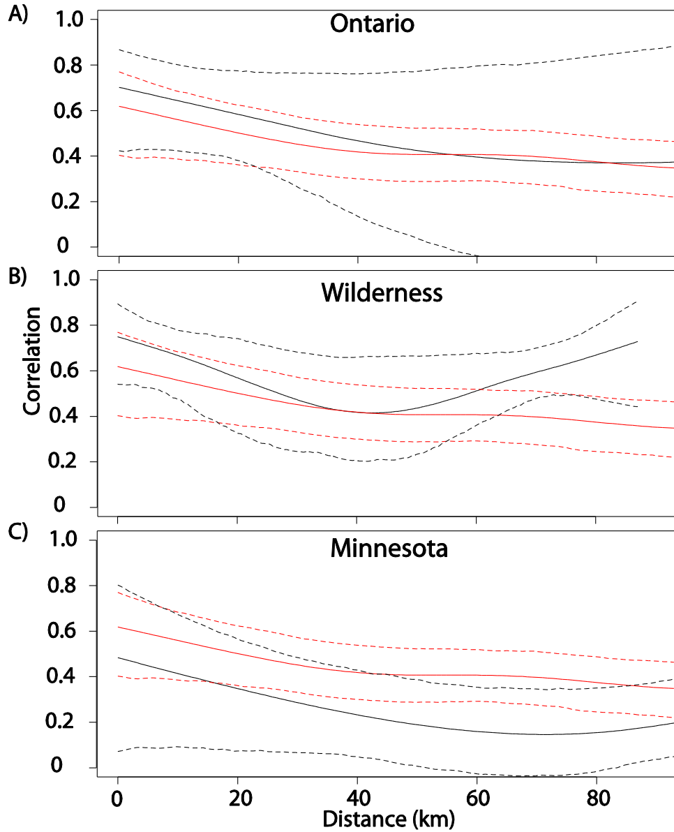
Figure 5: Spatial non parametric covariance functions (SNCF) for the different management zones in the BLL. Each management zone (black) is represented individually on separate graph (A, B, C) with their 95% confidence interval (dashed lines) and overlaid with the SNCF calculated for the entire BLL (red).
