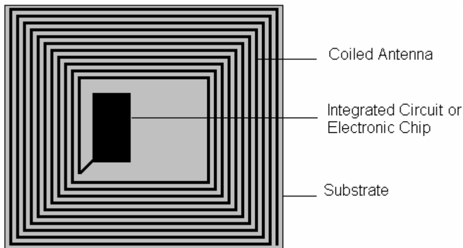
Figure 1. Basic components of an RFID tag (based on the description given by Gearoid, 2003).
