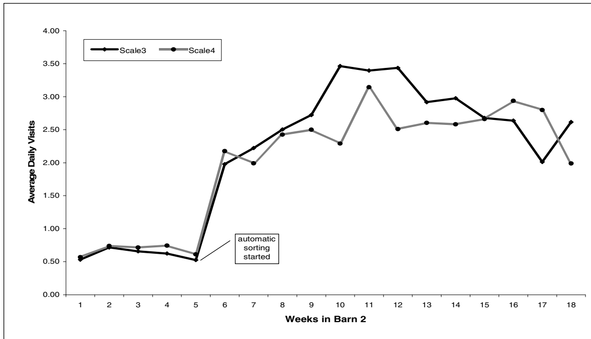
Figure 5. Trend of the estimated average daily visits (ADV) per pen in barn 1 (A) and barn 2 (B) computed weekly showing the differences in ADVs in all pens before and after automatic sorting was started and, in barn 1, when the RFID antenna was not properly placed.
