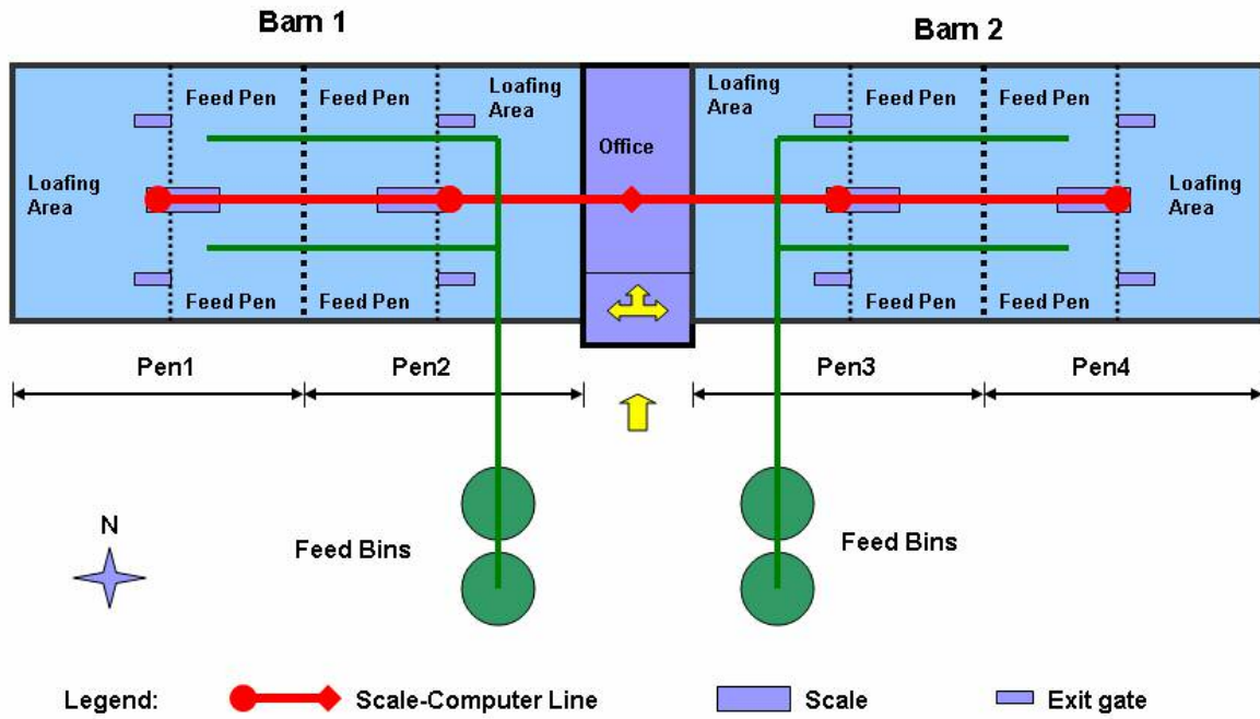
Figure 1. Farm lay-out.
