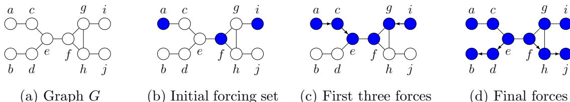
Figure 3.1: Standard zero forcing game example
