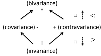
Figure 4.9 Polarity Lattice.
